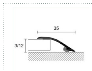
PERFIL DE REMATE AUTOADHESIVO* SELF-ADHESIVE FINISH PROFILE* L: 270cm.
